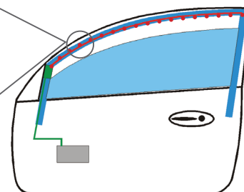
Two methods of protection provided by a single CSA ODS sensor strip.
